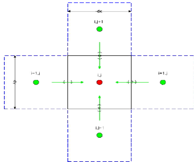
Fig. 3 Basic grid used for the FDM approach
