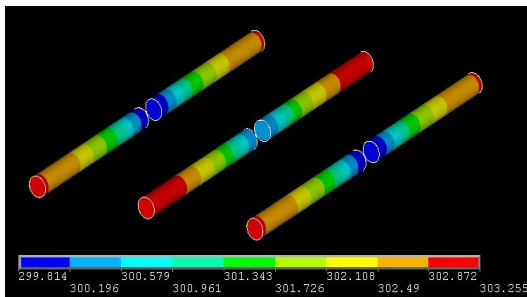
Fig. 4. Rod diagram of the results using ANSYS
