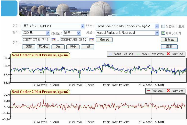
Fig. 2. Normal state condition of Seal Cooler 2 Inlet Pressure.
