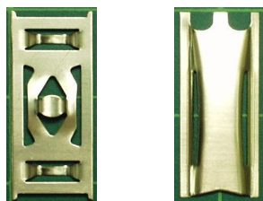
Figure 1 KAERI's SG springs(Left: Opt. H; Right: Doublet).
