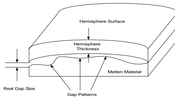
Fig. 3 A schematic of a sample 1.
