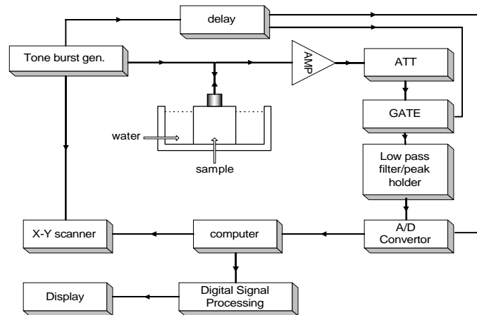
Fig. 2 Blocks diagram of the scanning acoustic microscope.
