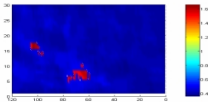
Fig. 7 Sectional image reconstructed with a single frequency
