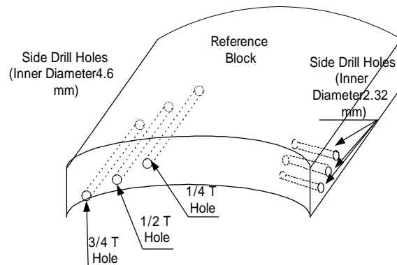
Fig. 6 A schematic of a sample 2 (Reference Block).
