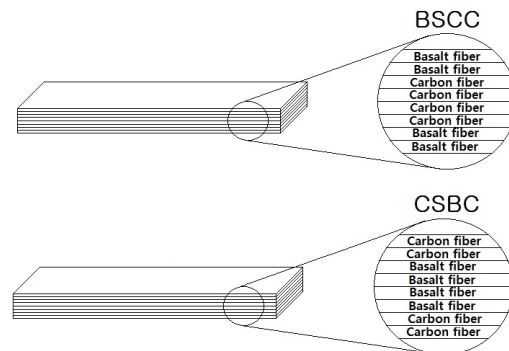
Fig. 1. Stacking sequence of composites
