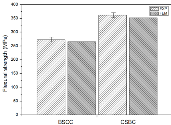
Fig. 3. Comparison of flexural strength of experiment and finite element results
