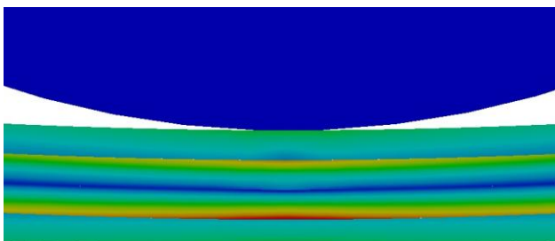
Fig. 5. Stress distribution of BSCC composite
