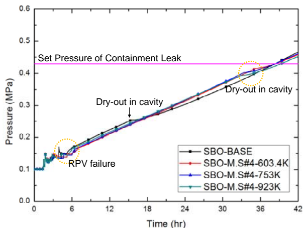
Fig. 3. Containment pressure of SBO cases
