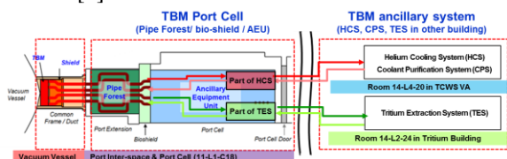
Figure. 1 Schematics of HCCR-TBS
