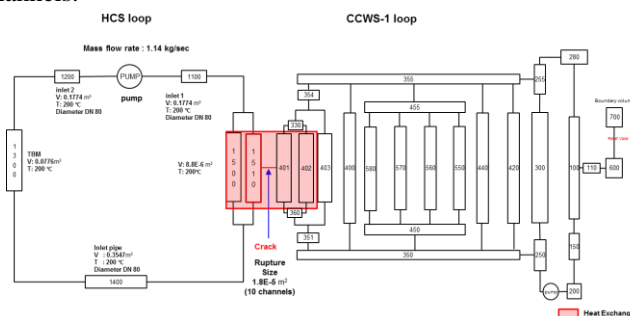
Figure. 3 HCS + CCWS-1 nodalization
