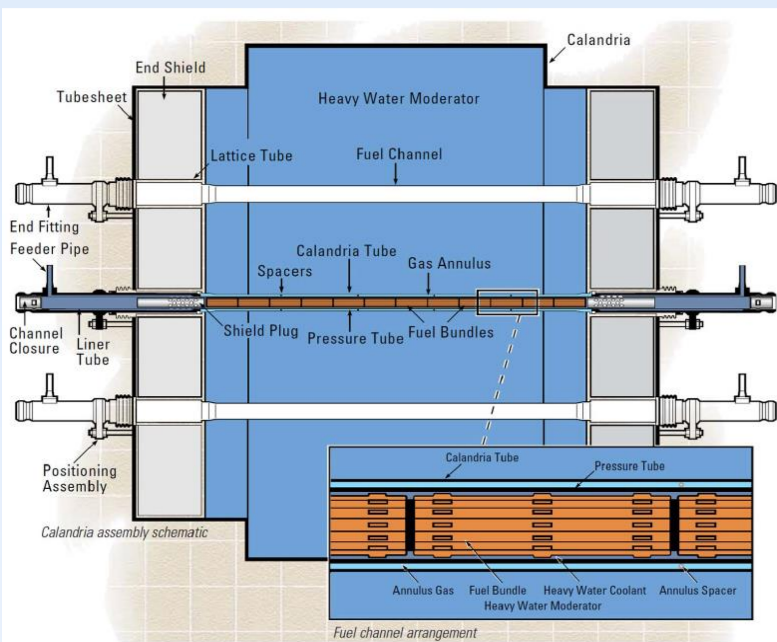
Fig. 1. CANDU Reactor Structure
