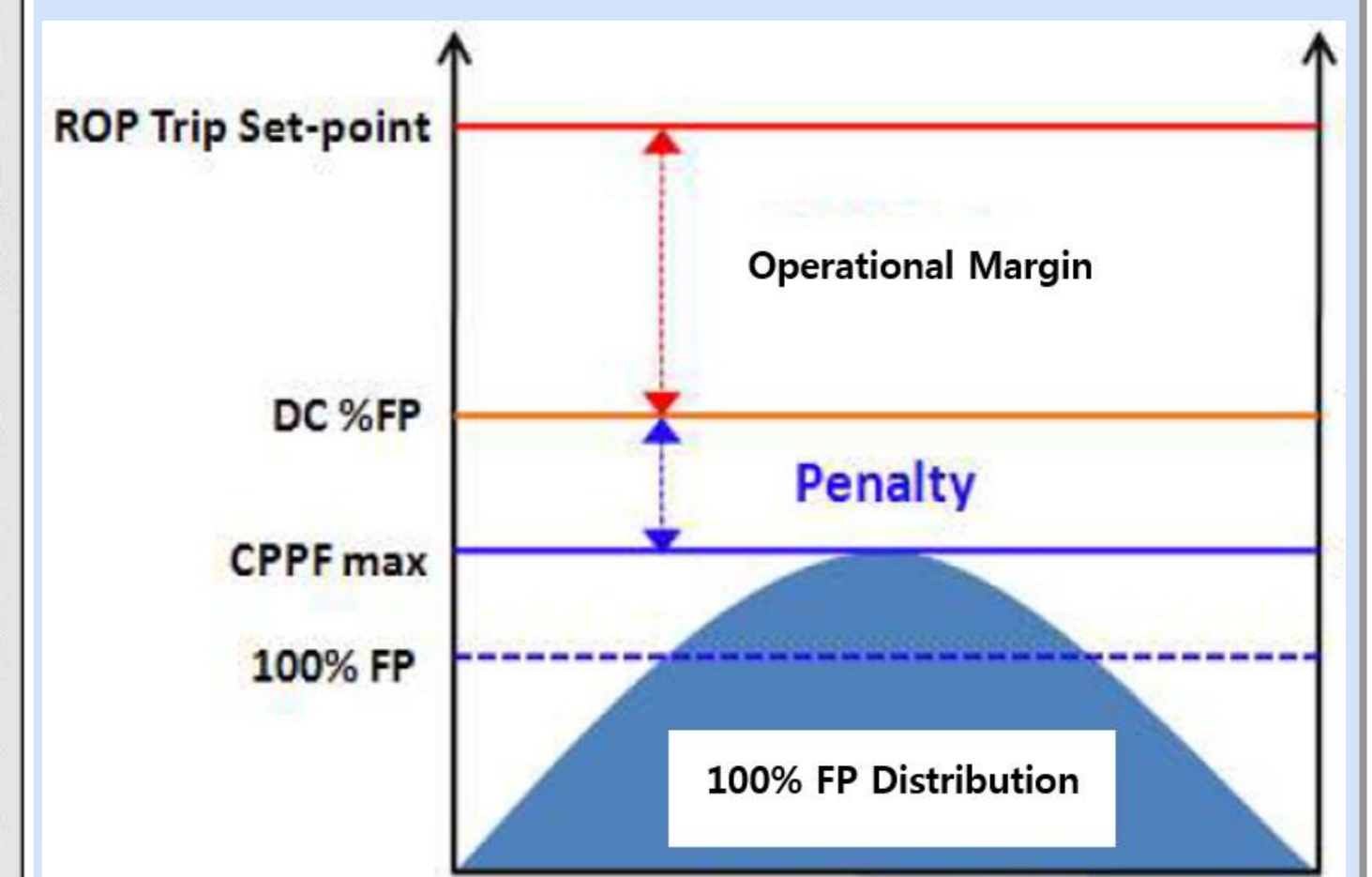
Fig. 6. CANDU6 ROP Trip Set Point and Operational Margin
