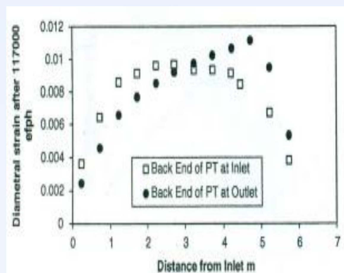
Fig. 3. Comparison of Diameter Profiles along Pressure Tube with Two Loading Categories
