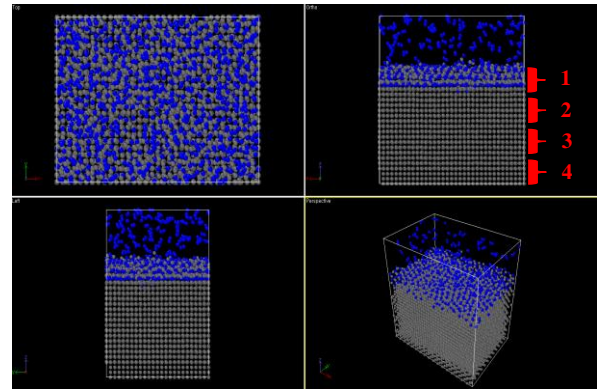
Figure 2. Final state of the Ni/Oxygen structure (Grey : Ni, Blue : Oxygen)
