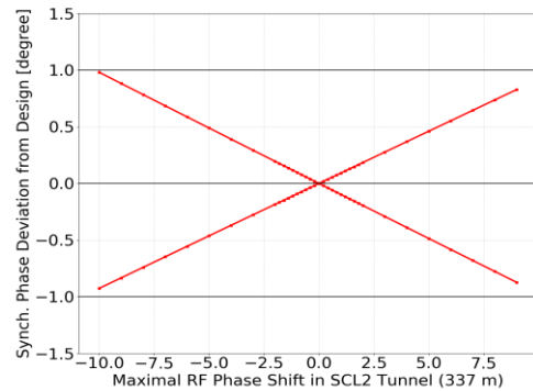
Fig. 1. Synchronous phase deviation due to RF phase shift in SCL2 tunnel.
