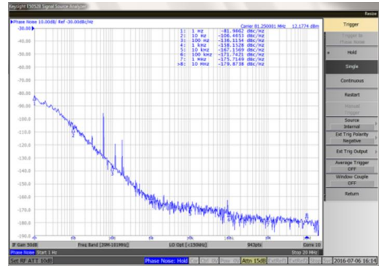
Fig. 5. The measured phase noise at 81.25MHz PLO output: RMS jitter was about 200 fs, and phase error was 0.006°. It means that the results satisfy the phase stability requirement of \pm 0.3^\circ on the temperature-controlled reference line with \pm 0.5^\circ\text{C} .
