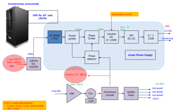
Fig. 4. Block diagram of master oscillator for RF reference clock generation.
