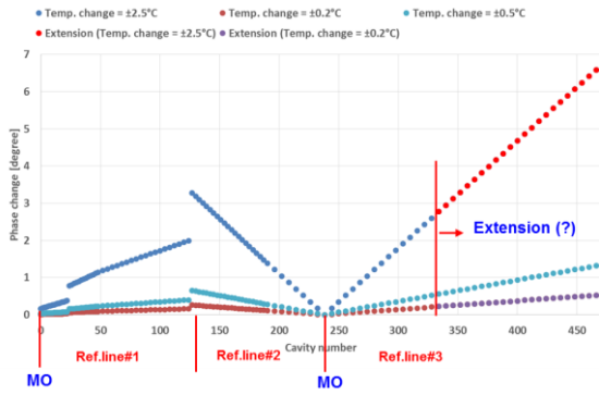
Fig. 3. Phase change (“degree” corresponds to the cavity RF frequency) due to temperature change for each of the cavity along the linac.
