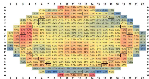
Fig. 8. Ratio of Lifetime Average Fast Flux (> 1MeV) against Time-Average Model for Wolsong 2
