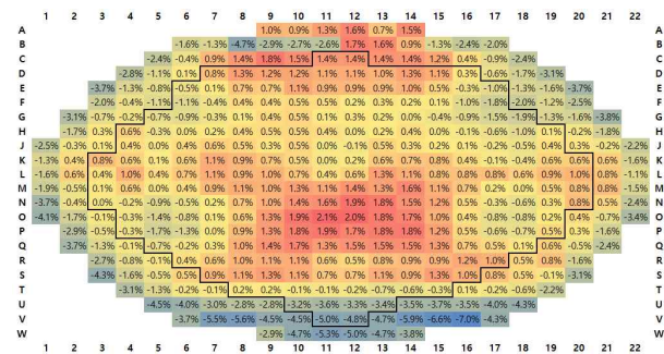
Fig. 9. Ratio of Lifetime Average Fast Flux (> 1MeV) against Time-Average Model for Wolsong 3
