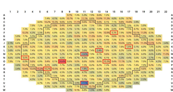
Fig. 6 PTDC Ratio of Site-specific Estimation vs. to RC-1980 Estimation for Wolsong Unit 4(6000EFPD) Pressure tube diametral creep is commonly the highest in the central core, where the fast neutron flux is the highest as shown in Fig. 7[2]. However, PTDC Ratio of Wolsong 2, 3 & 4 have different trend, because site-specific
