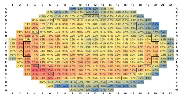
Fig. 10. Ratio of Lifetime Average Fast Flux (> 1MeV) against Time-Average Model for Wolsong 4
