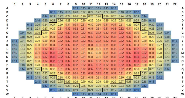
Fig. 7. Time-Average Fast Flux (> 1MeV, 10 14 )
