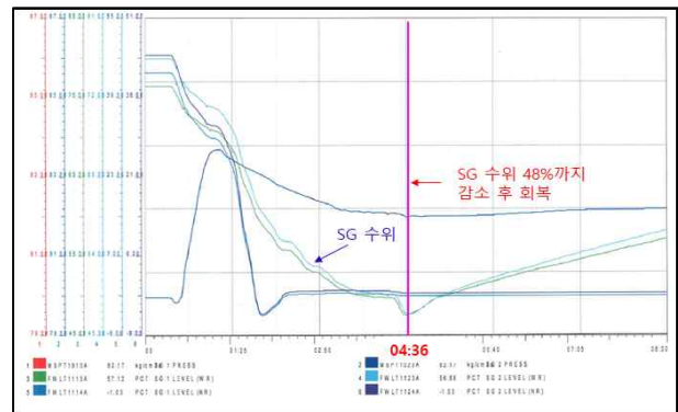
Fig. 1. CASE A : Manual insertion of the control rods
