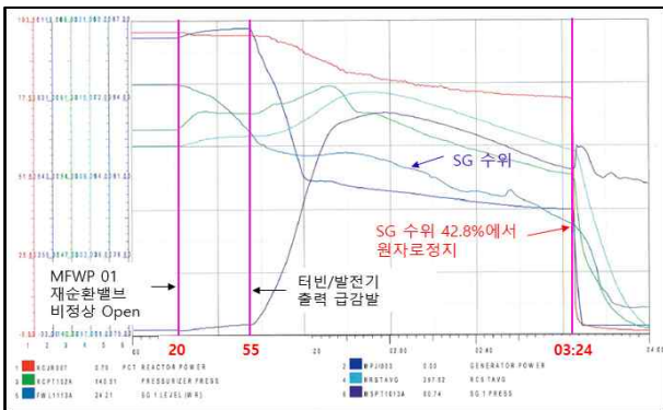
Fig. 3. CASE A : Sharp decrease in turbine power to 400MW at 64% (WR) of the steam generator level
