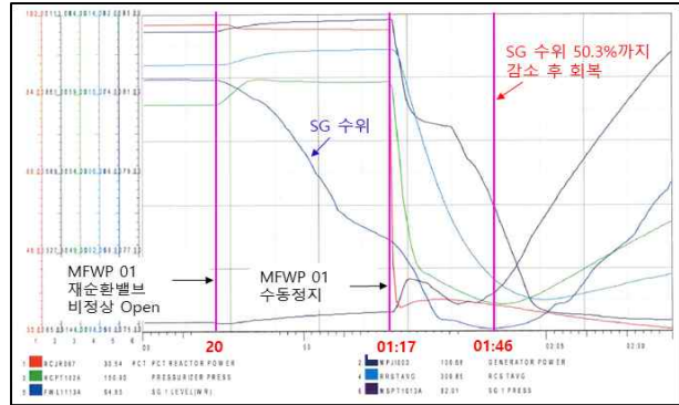
Fig. 4. CASE B : Manual shutdown of the main feedwater pump at 60% (WR) of the steam generator level
