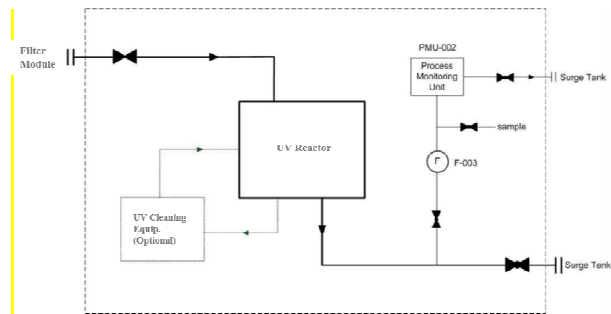
Fig. 2. Detailed design of UV reactor module
