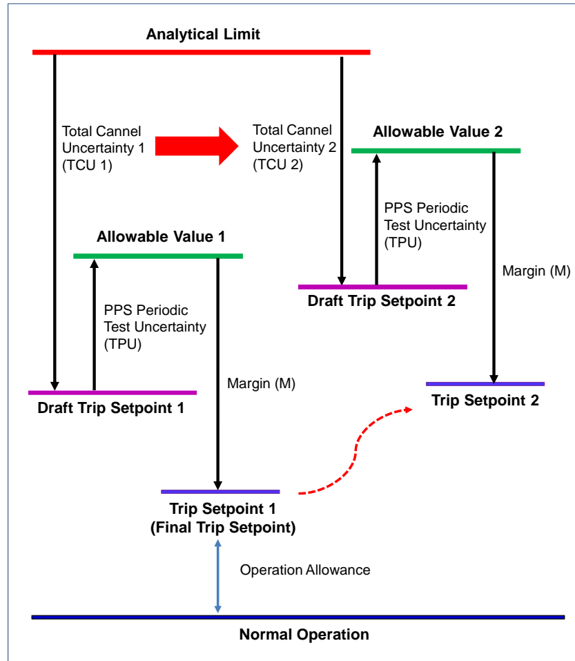
Fig. 1. PPS trip setpoint evaluation due to instrument uncertainty change
