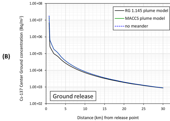
Fig.1. (A) Ground air concentration ( \text{Bq}\cdot\text{s}/\text{m}^3 ) and (B) center ground concentration ( \text{Bq}/\text{m}^2 ) of Cs-137 for ground release (mean value)
