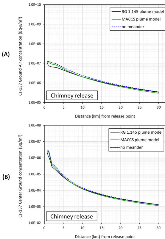
Fig.2. (A) Ground air concentration ( \text{Bq}\cdot\text{s}/\text{m}^3 ) and (B) center ground concentration ( \text{Bq}/\text{m}^2 ) of Cs-137 for the release through chimney (mean value)
