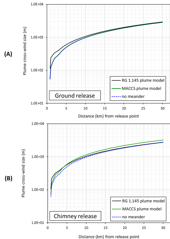
Fig.3. Plume cross wind size (m) of (A) Ground release and (B) chimney release (mean value)
