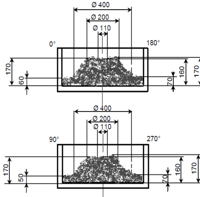
Fig. 6. Height of the debris in the catcher as measured along two radial positions after the test
