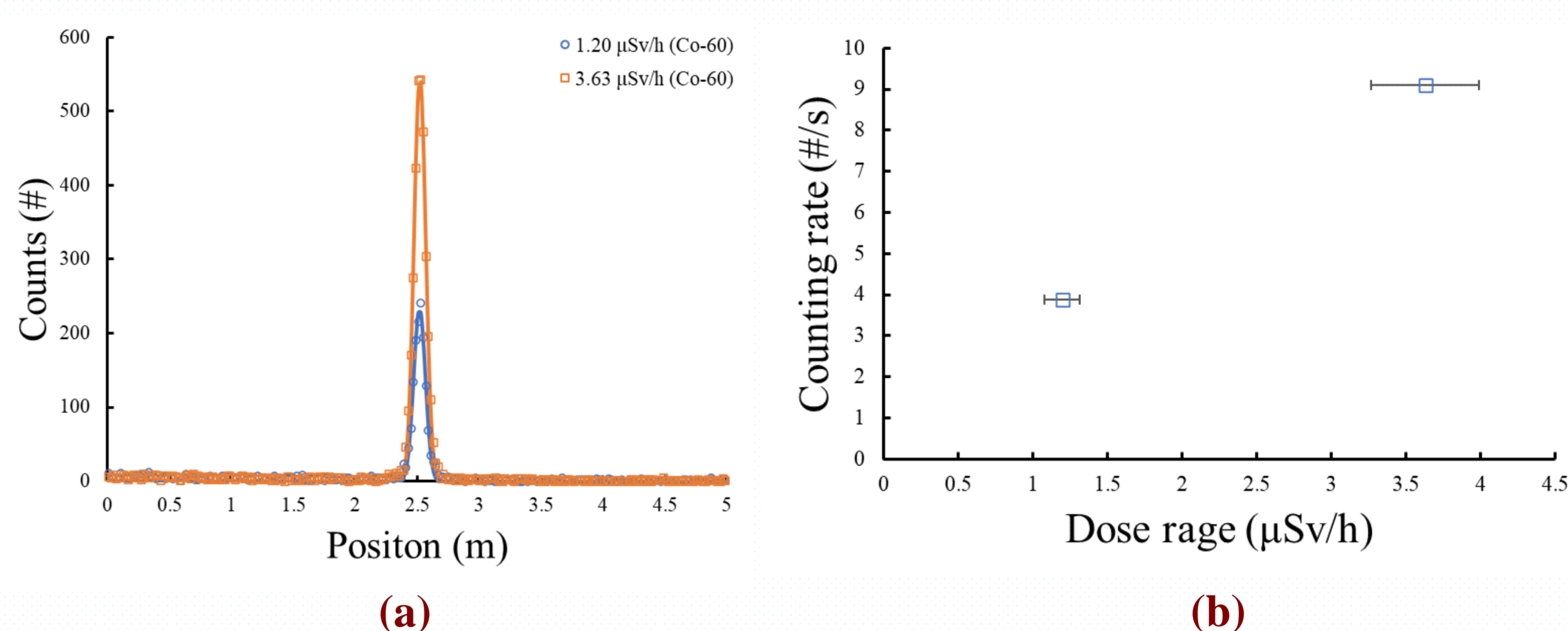
Fig. 2. (a) Measured position spectra and fitted Gaussian curves for non-collimated Co-60 gamma-ray sources located at 2.5 m. (b) Dose response of the position-sensitive PSOF bundle detector.
