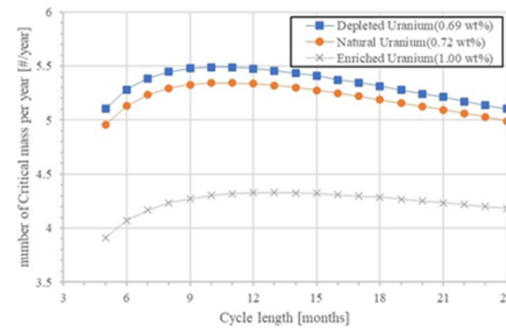
Fig 3. Number of critical plutonium sphere produced per year versus the enrichment of U-235 and the cycle length with one month break after burnup.
