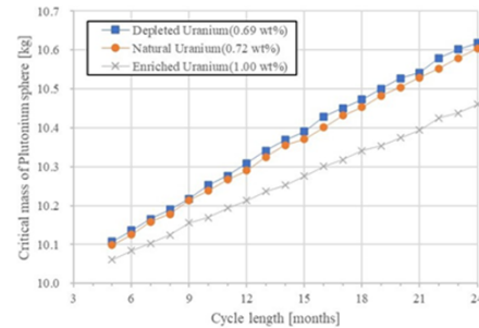
Fig 2. Change of critical mass of plutonium sphere versus the enrichment of U-235 and the cycle length with one month break after burnup.
