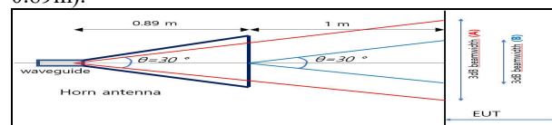
Figure 3. horn antenna 3dB Beamwidth
