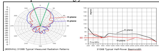
Figure 2. 3106B Antenna(200MHz~1GHz)
