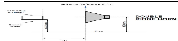
Figure 1. Antenna positioning
