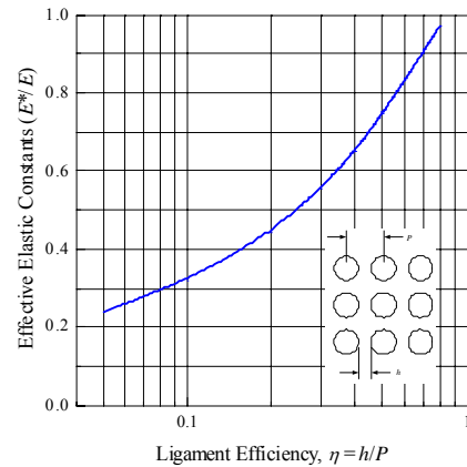
Fig. 5. Effective elastic constants of perforated shell with a square penetration pattern
