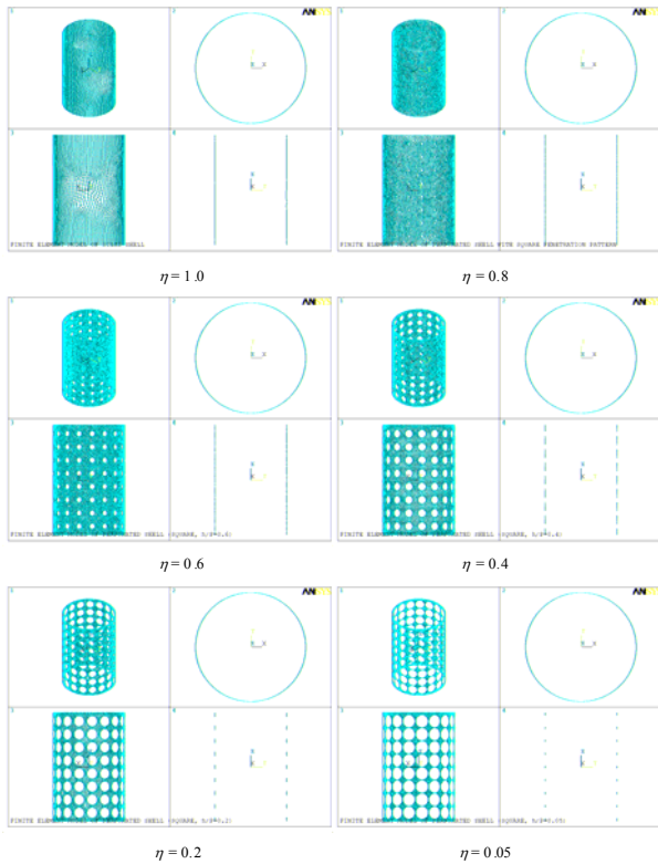
Fig. 3. Finite element models of solid and perforated shells with a square penetration pattern
