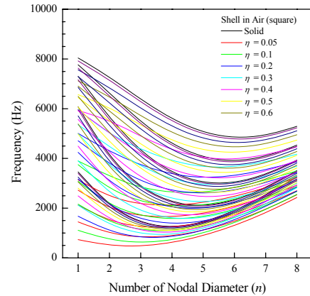
Fig. 4. Natural frequencies of shell in air for solid shell and perforated shells with a square penetration pattern
