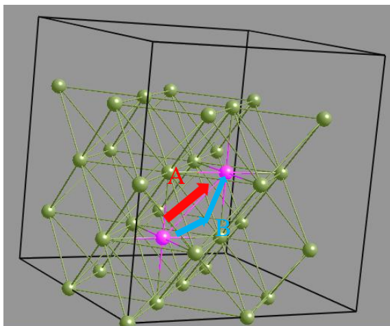
Fig 2. Calculation supercell (O-O(A), O-T-O(B))
