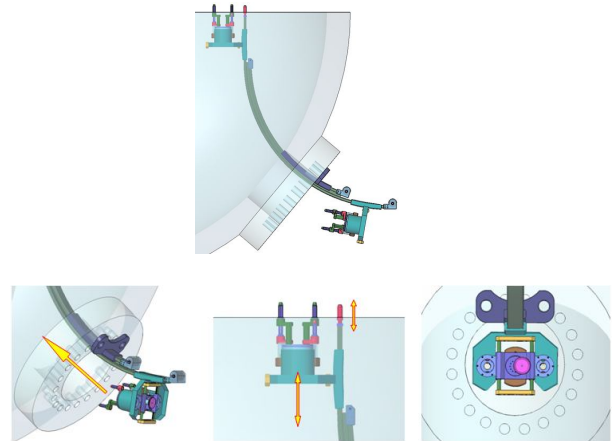
Fig. 5. Installation assisting equipment
